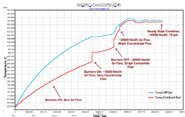
Figure 7. Steady state condition with 75 tph concentrate flow and 40,000 \text{ Nm}^3/\text{h} airflow rate as a function of time and temperature.
