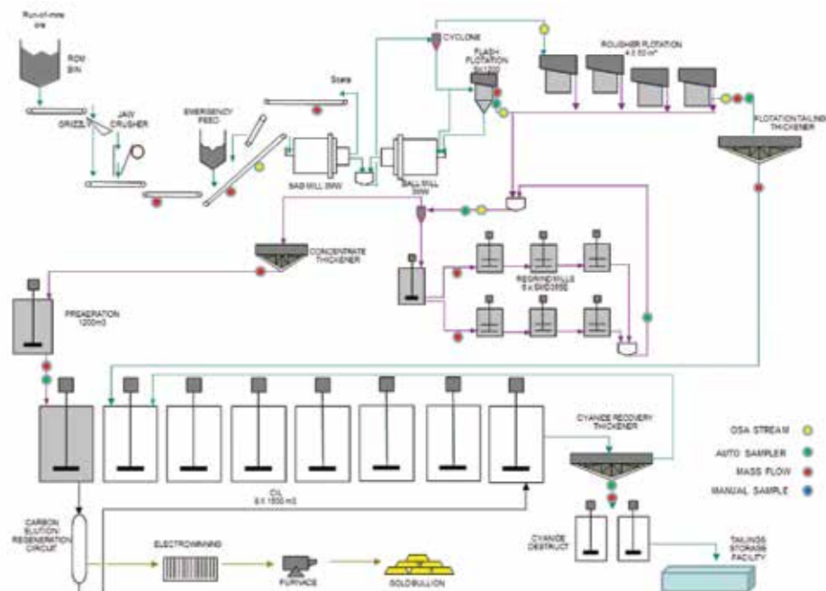
Figure 1 Haile processing plant flowsheet.
