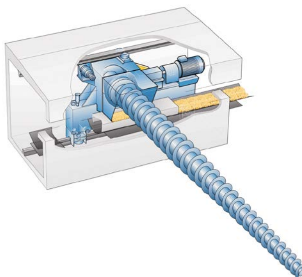
Cutaway view of the CantiScrew traveling screw reclaimer
