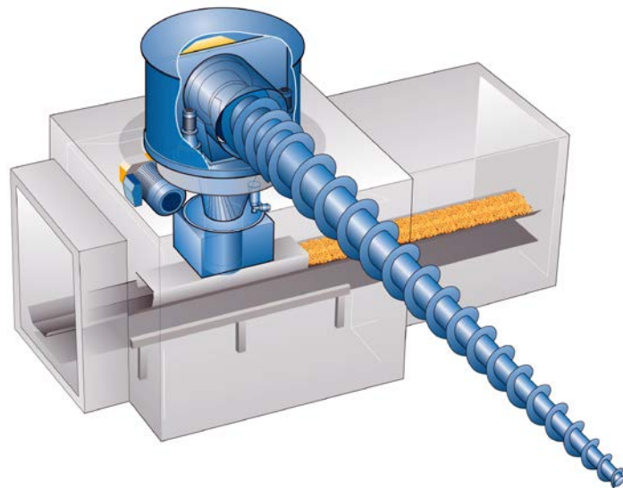
CenterScrew RCE slewing screw reclaimer with conical cantilever screw
