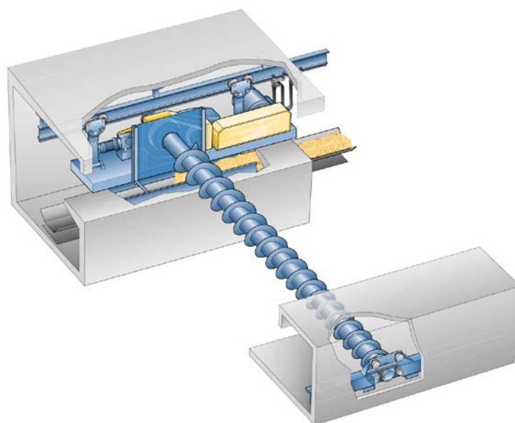
Cutaway view of the ParaScrew traveling screw reclaimer
