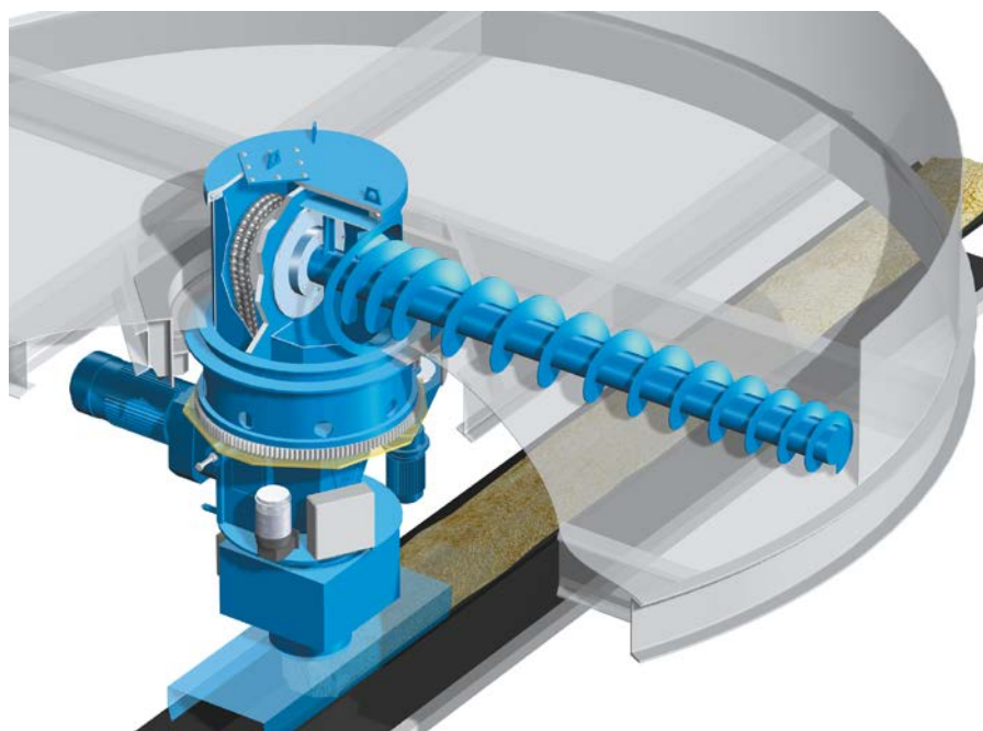
Cutaway view of PowerScrew slewing screw reclaimer
