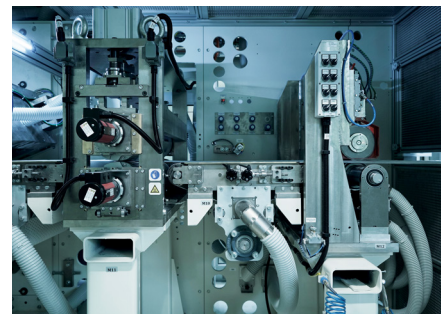
Core forming
