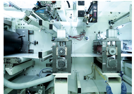
Production process ANDRITZ food pad eXcelle
