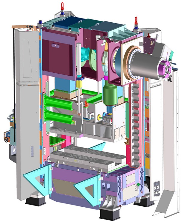
Details of the internal design of the machine, in particular the bionic structure
