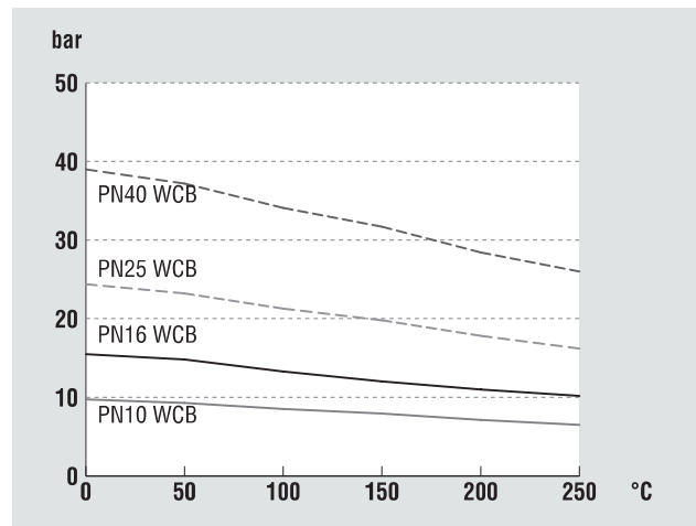
Carbon steel body (WCB)
