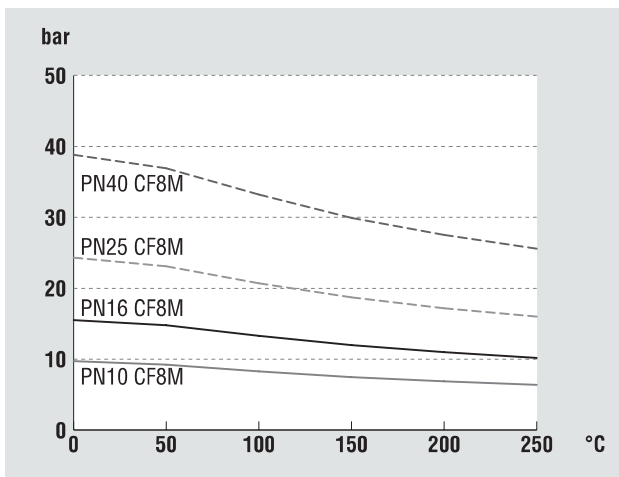
Stainless steel body (CF8M)
