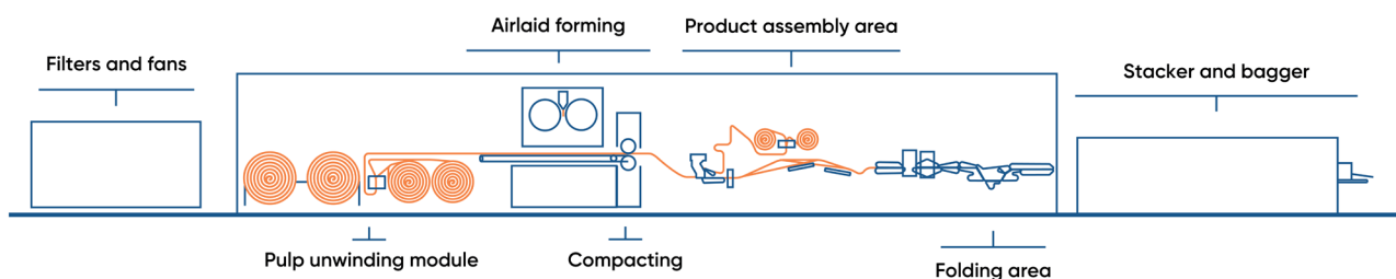
ANDRITZ Underpad Airloid eXcelle 2D-configuration
