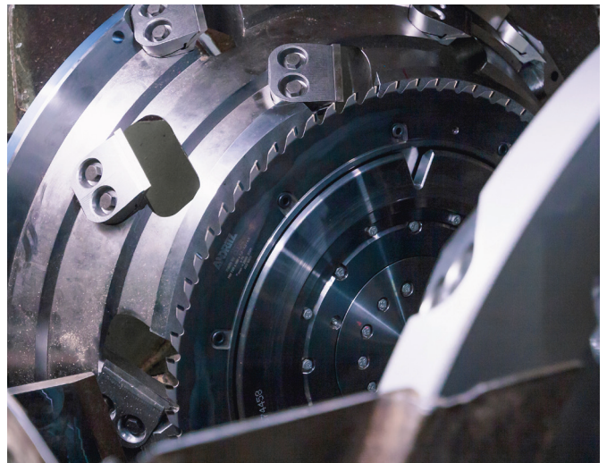
ANDRITZ sawblade installed on a PowerHead canter head
