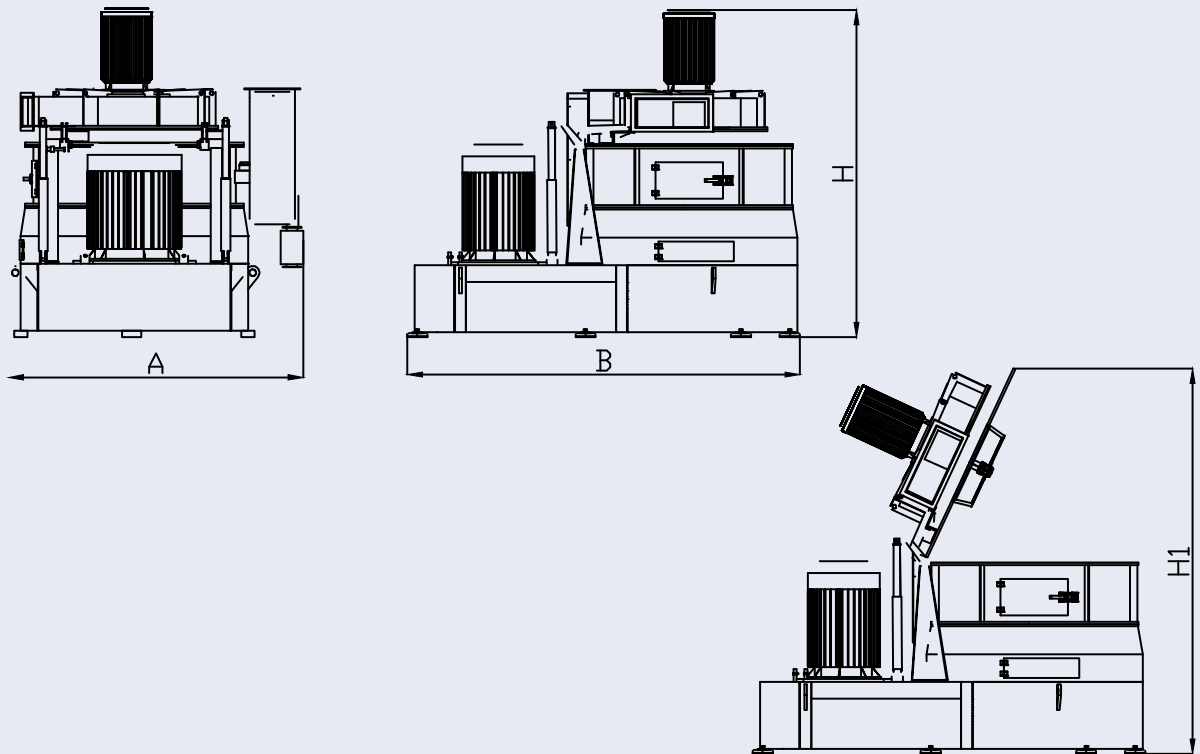
Dimensional sketch
