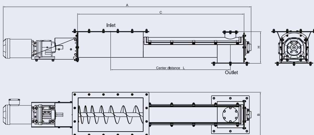
SF series screw feeder
