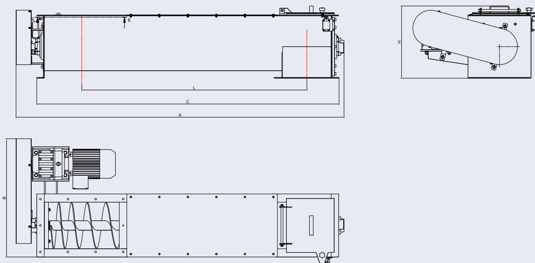
SFB300 screw feeder
