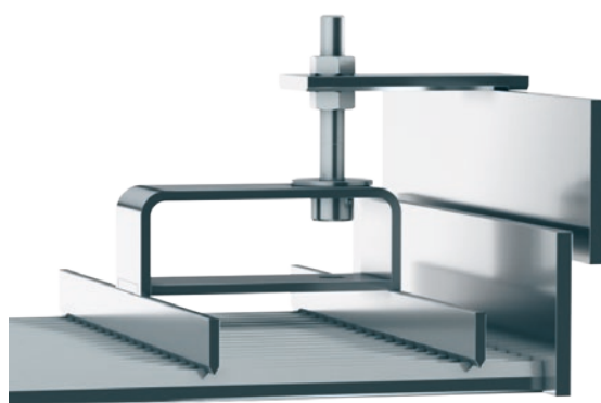
Ceiling fixation
