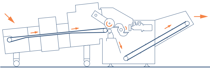
Starcut rotary cutter
