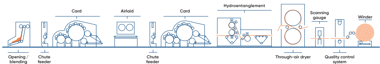
ANDRITZ neXline airlace hybrid line including airlaid forming unit, carding and hydroentanglement
