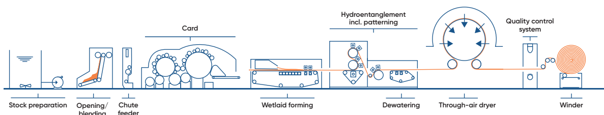
ANDRITZ neXline wetlace hybrid for carded-pulp wipes
