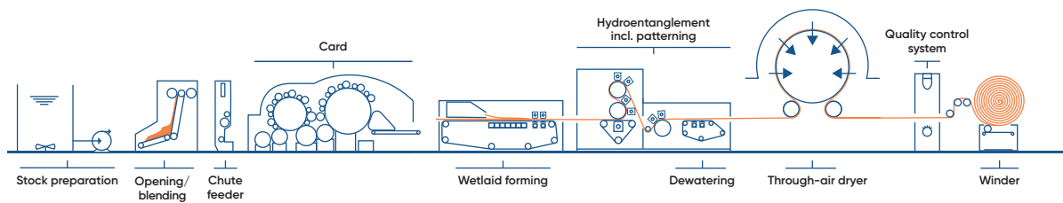
ANDRITZ neXline wetlace hybrid for carded-pulp wipes
