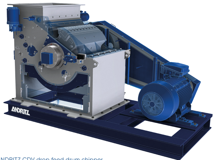
ANDRITZ CDV drop feed drum chipper
