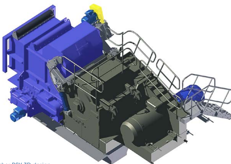
BioCrusher BSY 3D design
